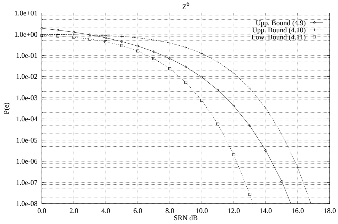
Figure 4.6: Upper and lower bounds to point error probability for \mathbf{Z}^6 .
