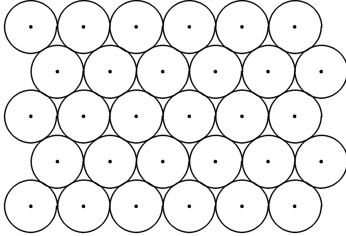
Figure 2.3: The optimal 2-dimensional lattice sphere packing
